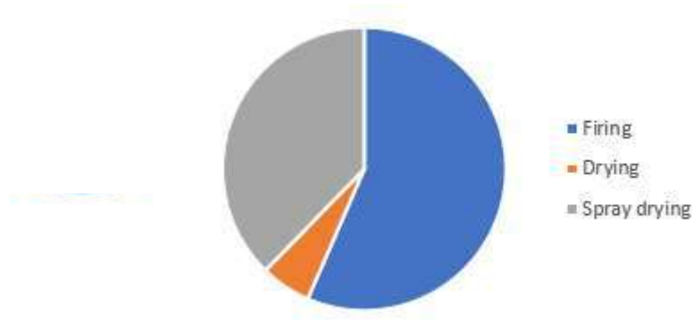
Figure 4 Distribution of thermal energy consumption during the tile manufacturing process [23]
